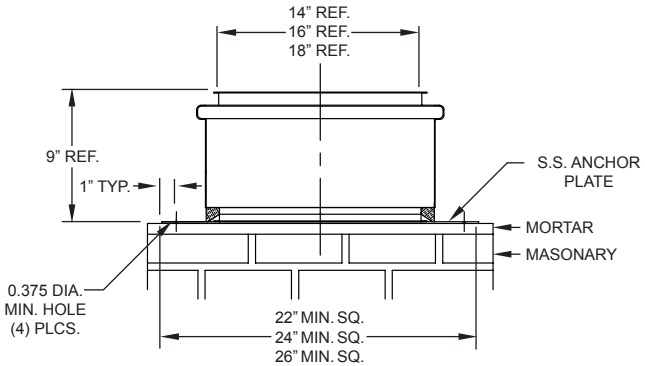
FIG. 15b 14TG, 16TG, AND 18TG ANCHOR PLATE
