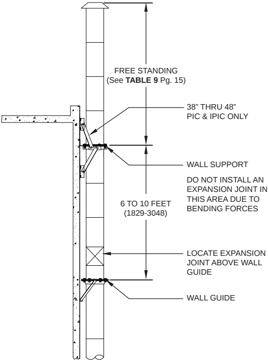
FIG. 6 - SPECIAL CONSIDERATIONS FOR GREASE DUCT ON OUTSIDE WALL
