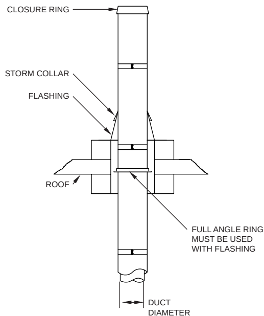
FIG. 7 - FULL ANGLE RING FOR LATERAL SUPPORT
