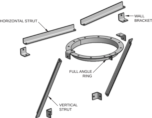
FIG. 5 - WALL GUIDE EXPLODED VIEW
