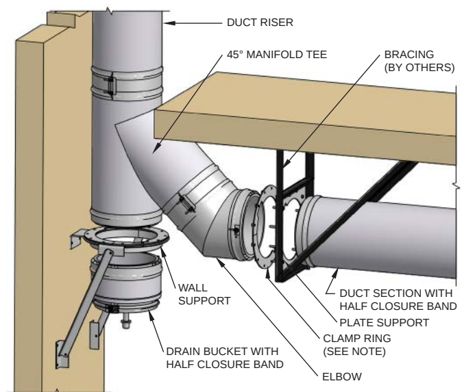
FIG. 16 - TWO-AXIS SUPPORT
