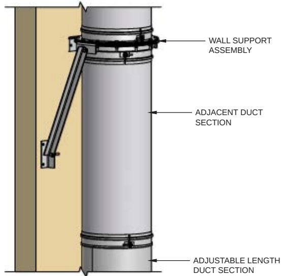
FIG. 9 - ADJUSTABLE LENGTH SUPPORTED WITH WSA
