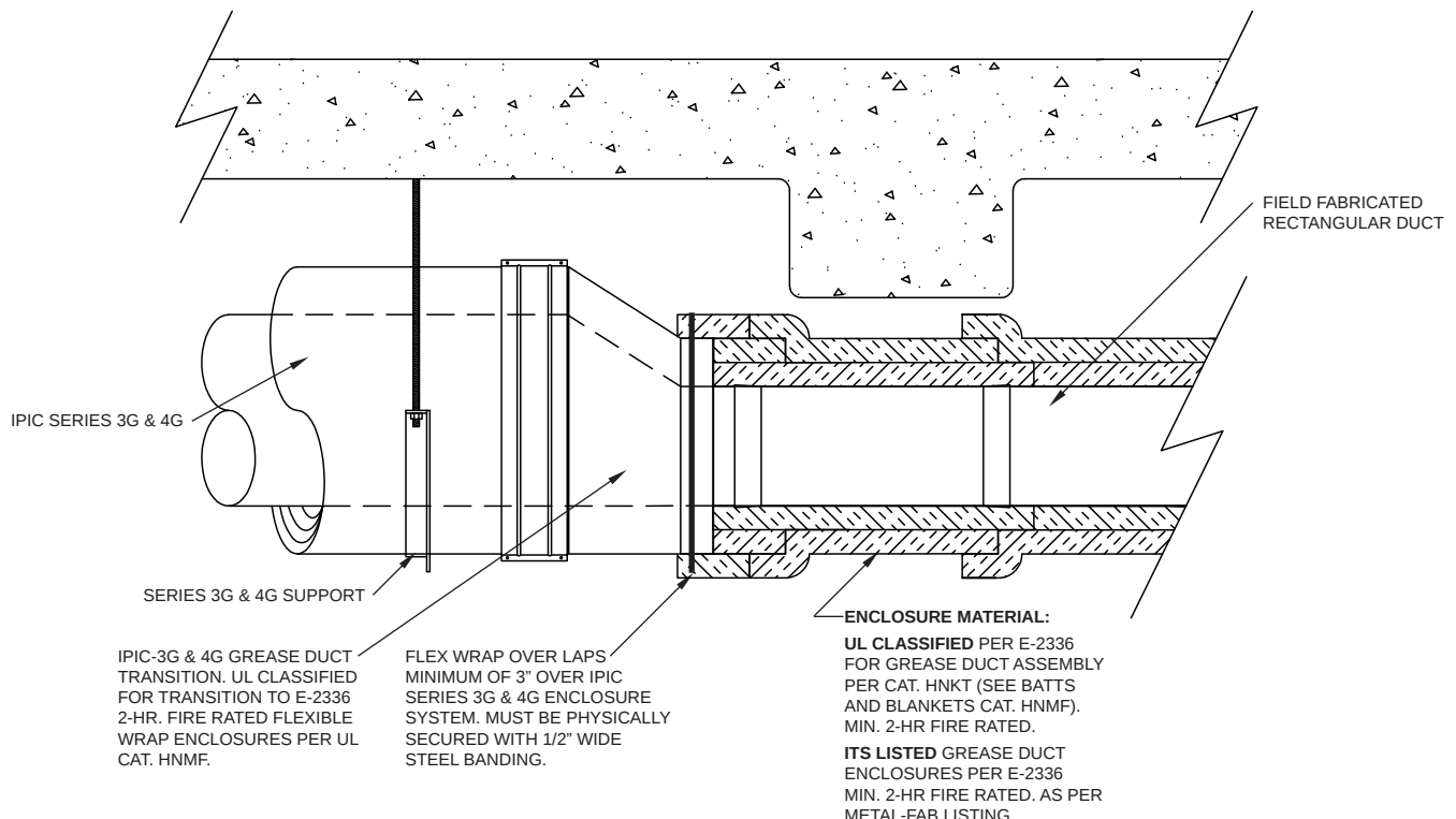
37-2 SERIES 3G & 4G TRANSITION TO FIRE RATED FLEXIBLE ENCLOSURE SYSTEM (Required For U.L. Classified Flexible Wrap Enclosure Systems)
