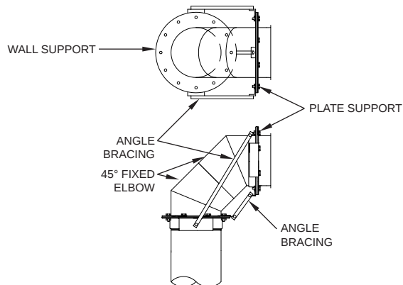
2-45° ELBOWS REINFORCED WITH WALL SUPPORTS
