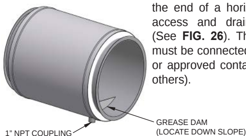
FIG. 26 - DUCT DRAIN TYPICAL LOCATION
