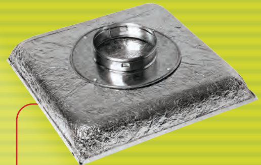
Collar Ring for Perforated Diffuser provides easy connection of flex duct 6", 8" 10", 12" or 14" dia.
