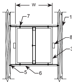
Top View MSCD Max. Size 196 sq. in. (W = 14-in. max.)
