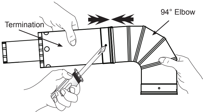
Install Horizontal Termination to Elbow - Figure 4
